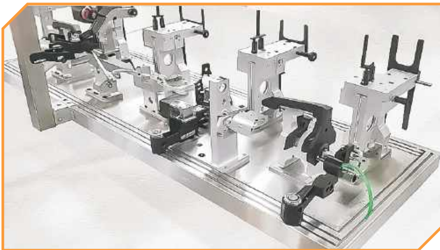
Đồ gá hàn (Welding fixture)
